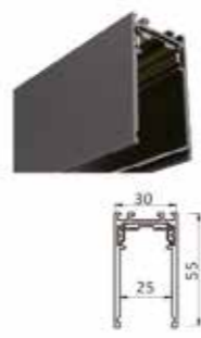
Surface mounted track (H55mm)
